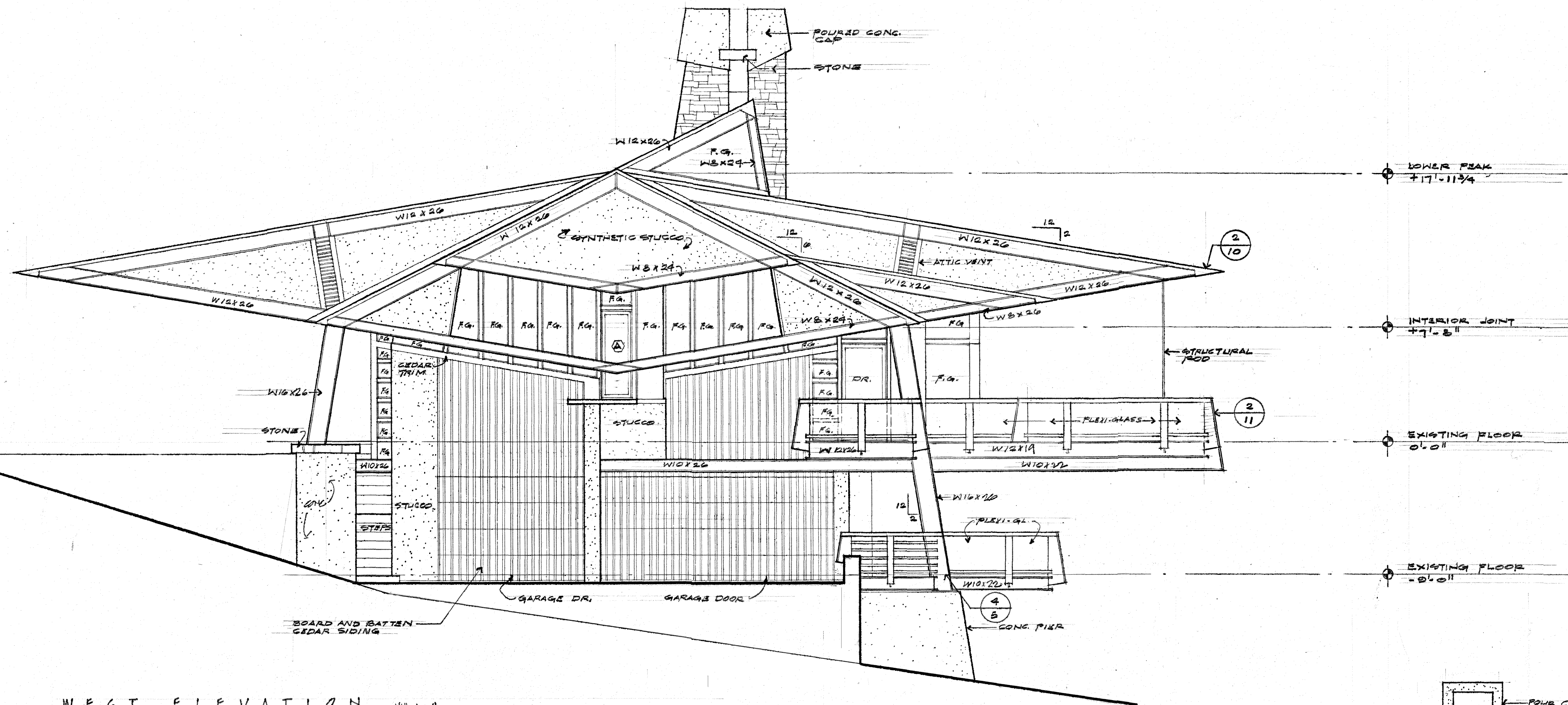
WEST ELEVATION 1/4"=1'-0"
