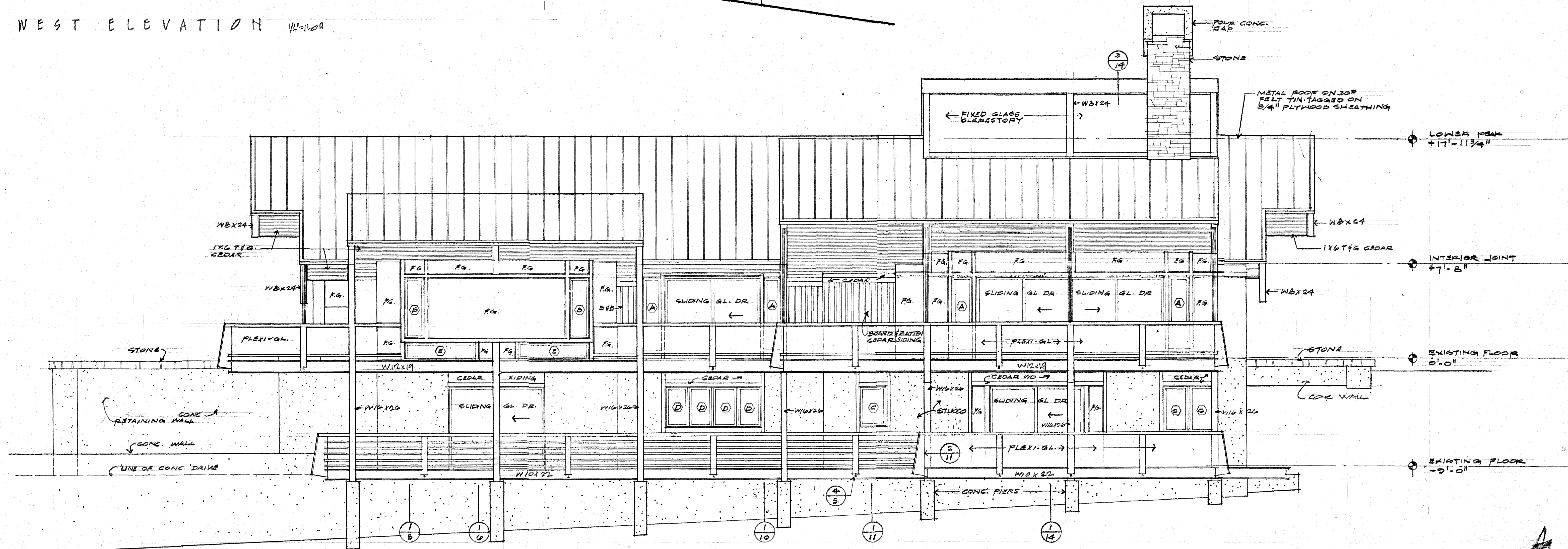
SOUTH ELEVATION 1/4"=1'-0"
